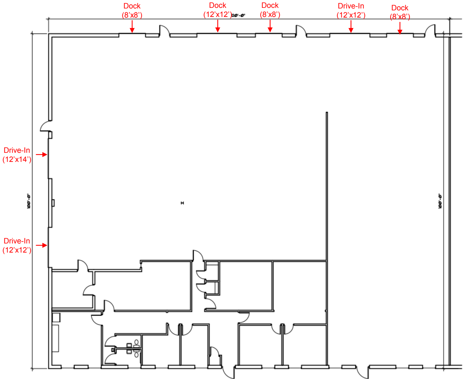
Floor Plan
